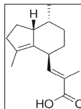
Fig. 1. Chemical structure of valerenic acid
